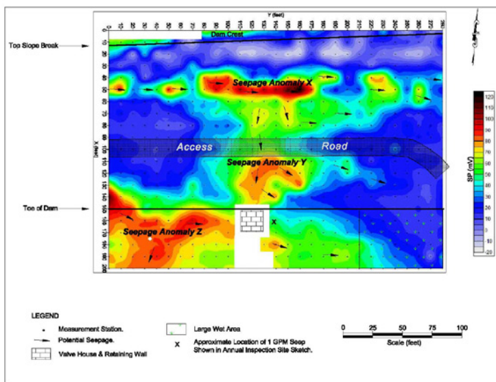
SP anomalies caused by seepage along earthen embankment and at toe of dam.
