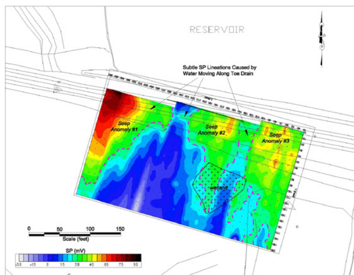
SP contour map showing three SP anomalies caused by seepage.
