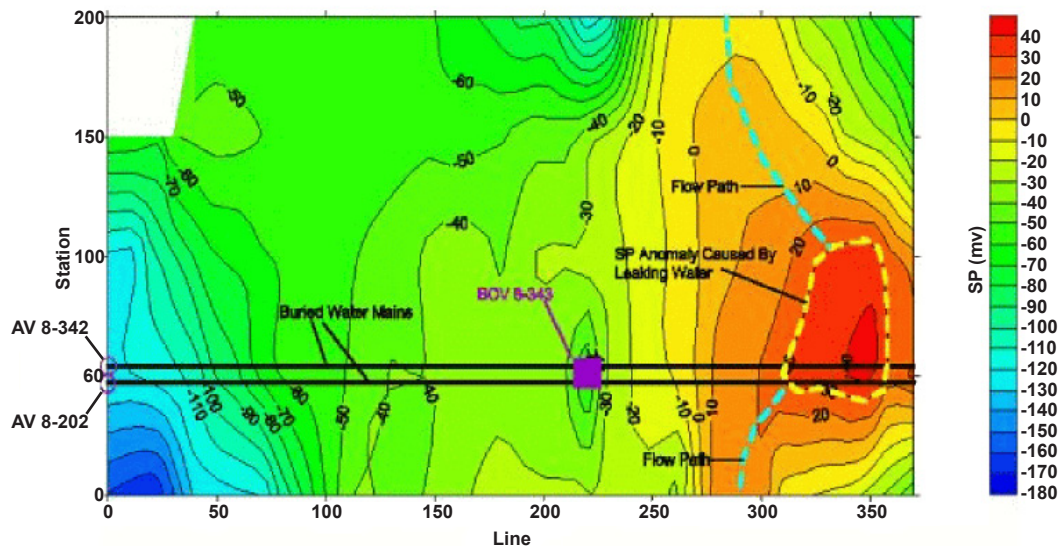
This SP contour map shows an anomaly (high SP measurements) caused by water leaking from a buried 36-inch water line at a major reservoir. The dashed light blue lines indicate the path of water movement.
