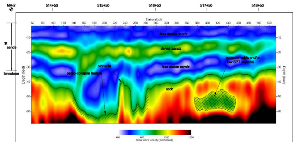
MASW-derived shear wave velocity profile showing soil stratification, bedrock surface, and karst, which includes a paleo-collapse feature (confirmed later from drilling), a pinnacle, voids, and/or low standard penetration test material within rock.
