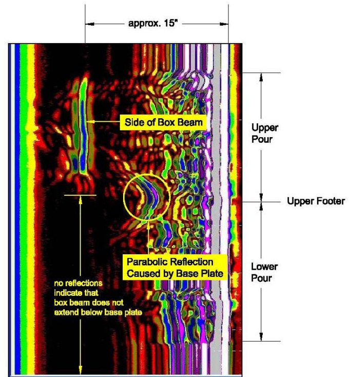
Using GPR to determine the depth of load-bearing column in footer
